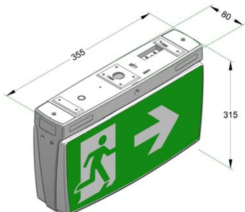
Dimensions (mm)
