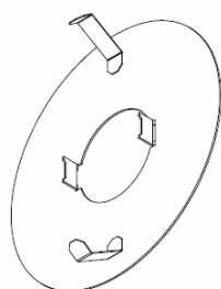
Optional adaptor plate for retro-fit of existing large head QI spinnings. P/N: PLIFE-ADP
