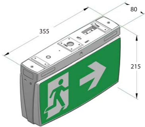
DIMENSIONS (mm)
